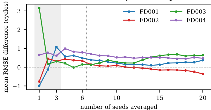
Fixed-order ARIMA hybrid minus plain
