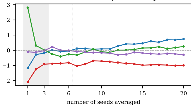
AIC-selected ARIMA hybrid minus plain
