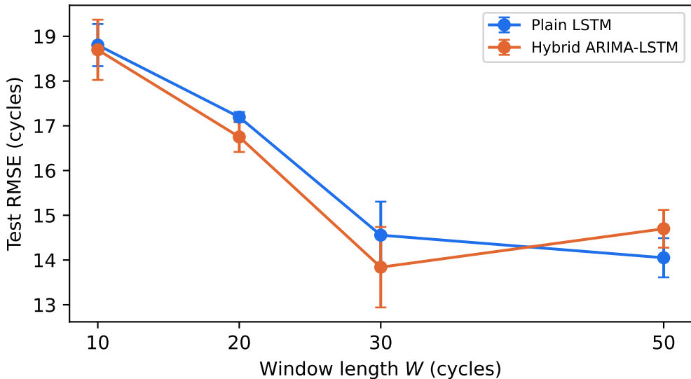
FD001: window length vs. RMSE, mean \pm std over 3 seeds
