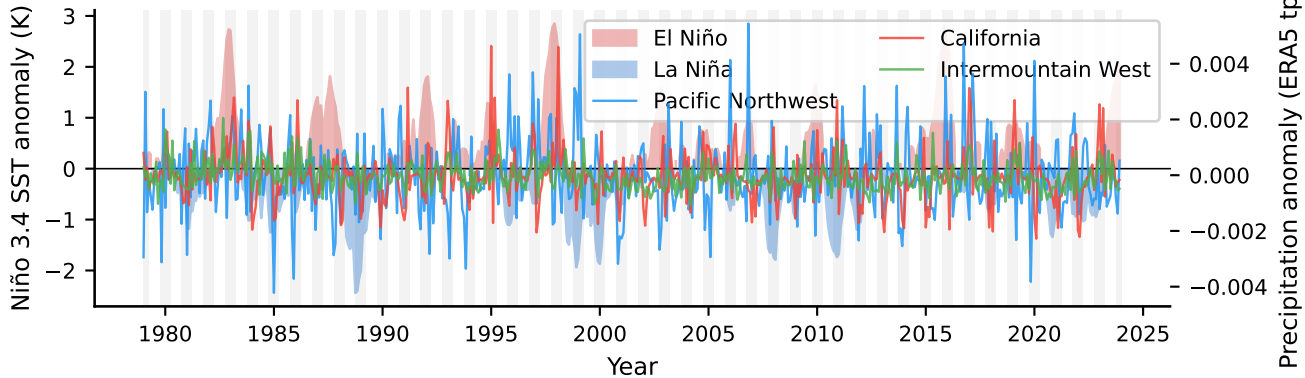
Niño 3.4 and regional tp anomalies (1979-01 — 2023-12); shading = inference months
