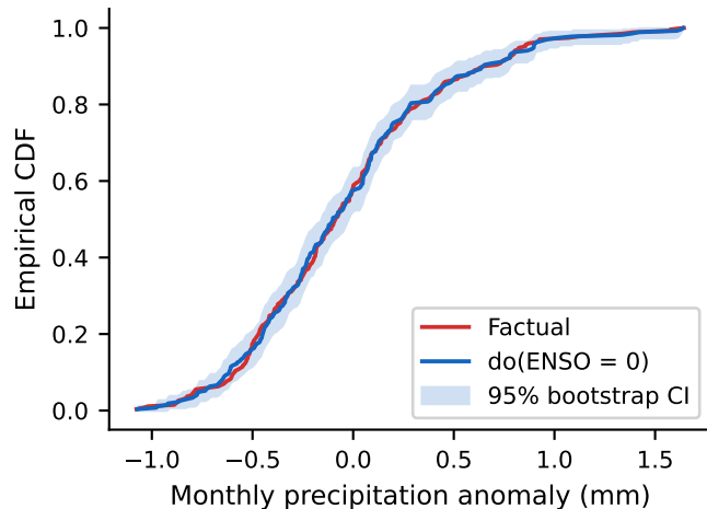
Counterfactual precipitation — Intermountain West
