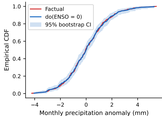
Counterfactual precipitation — Pacific Northwest
