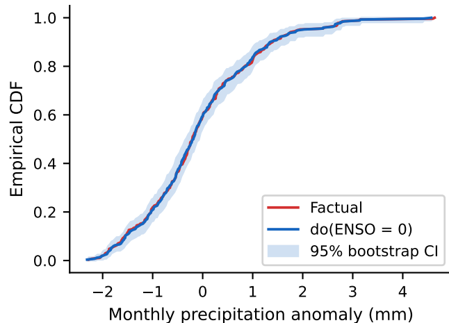
Counterfactual precipitation — California
