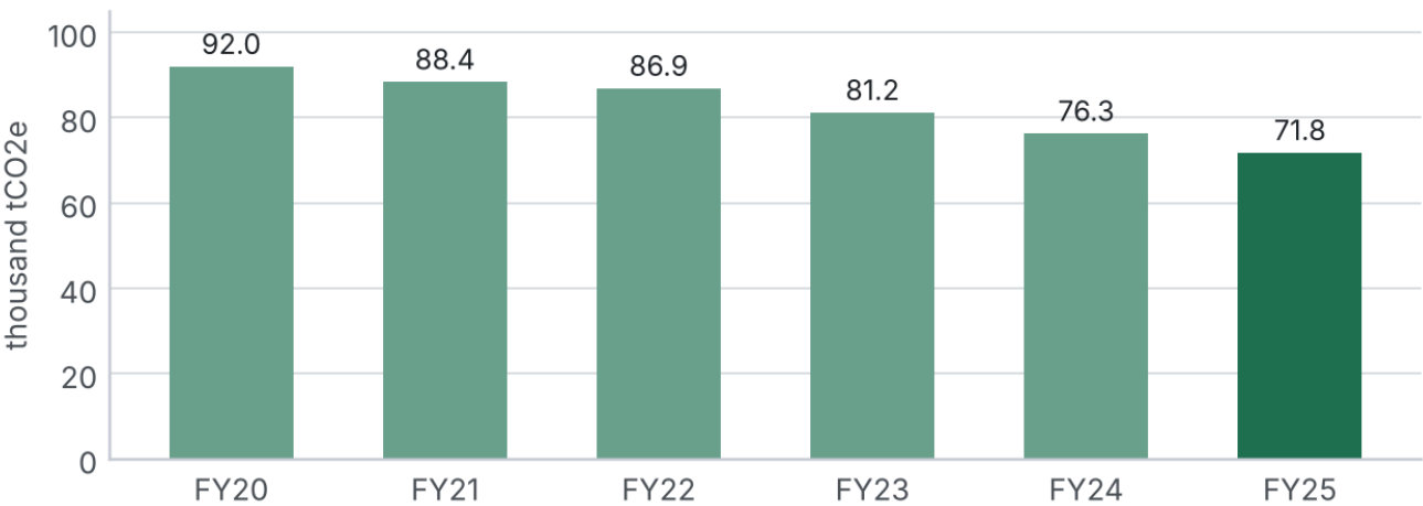
Figure 6.1 Scope 1 GHG emissions, FY2020 to FY2025 (thousand tCO 2 e).
