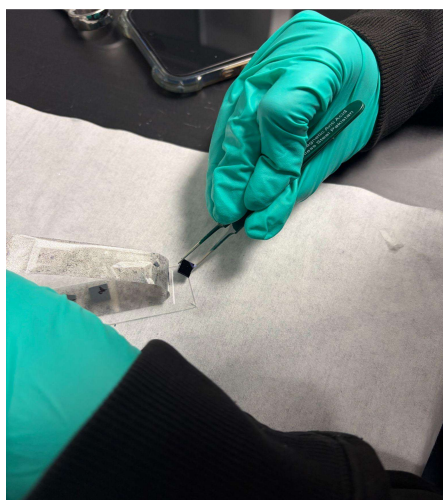
Transfer to SiO 2 Chips
