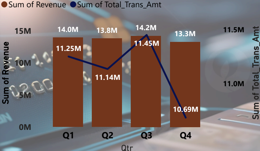
Sum of Revenue and Sum of Total_Trans_Amt by Qtr
