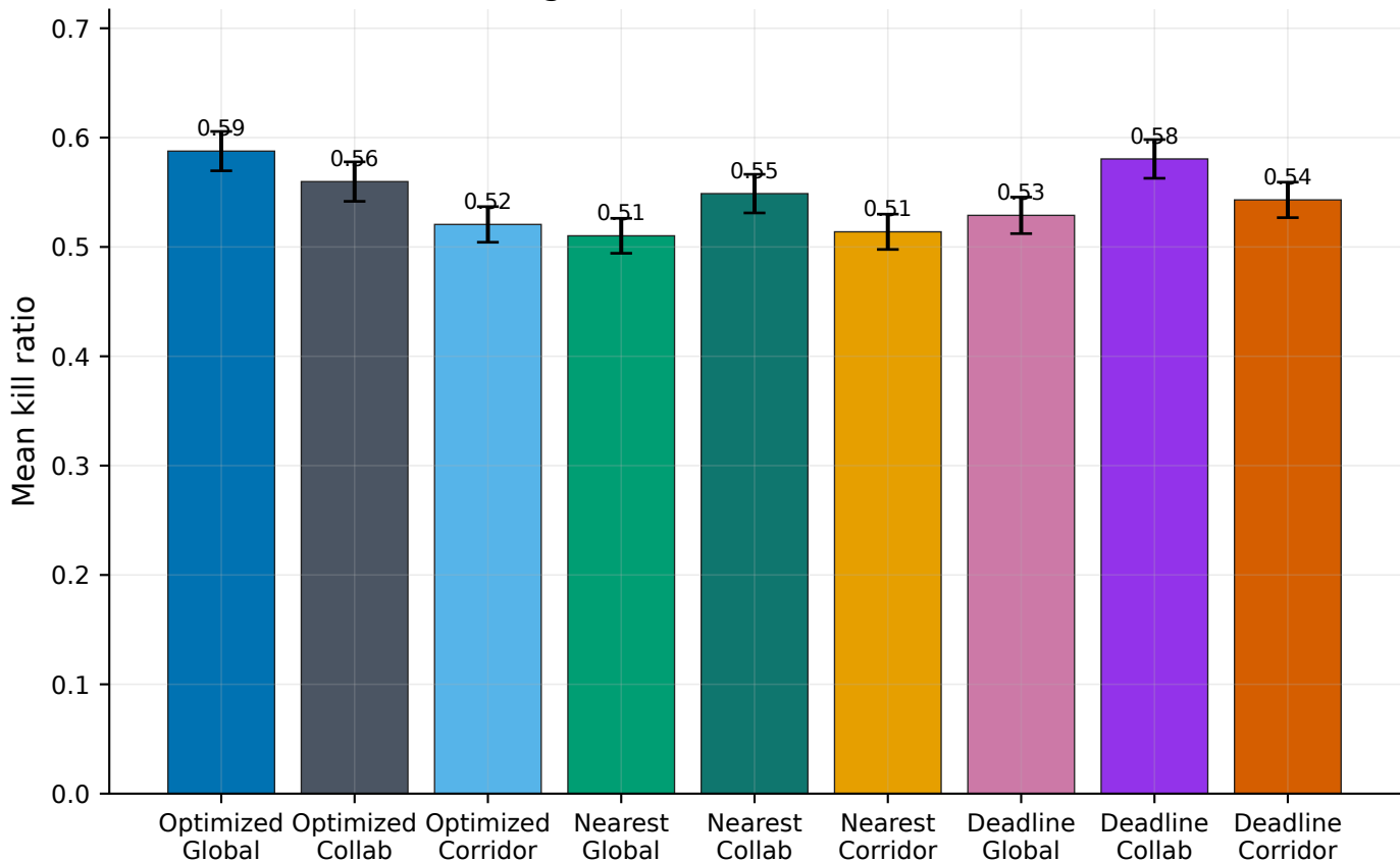
Average Fraction of Attackers Killed
