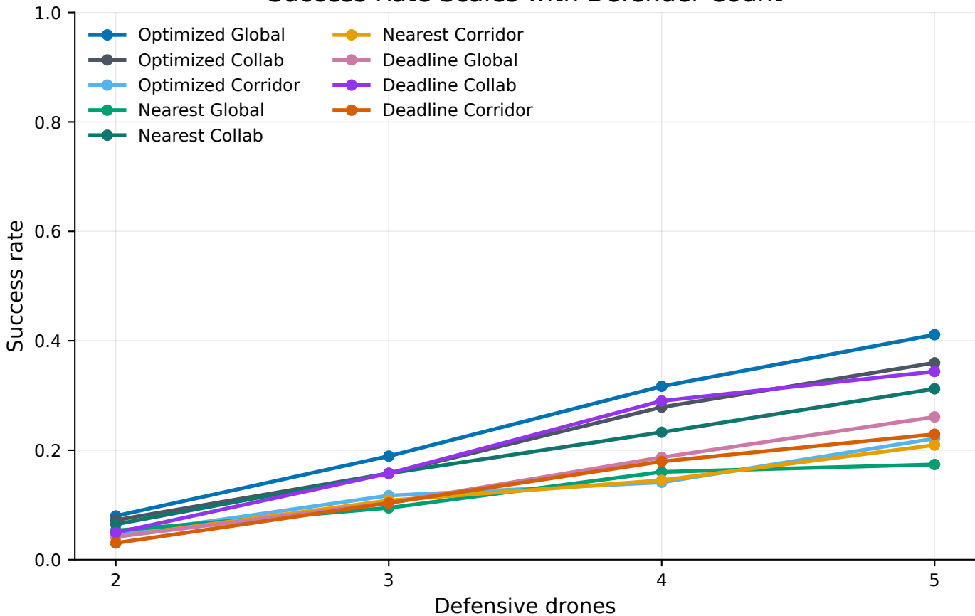
Success Rate Scales with Defender Count
