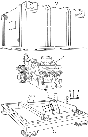
Figure 1. Engine and Container Assembly.
