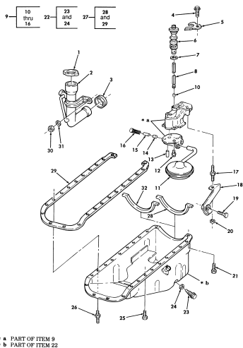
Figure 4. Engine Oil Pan, Pump, and Filler Tube.
