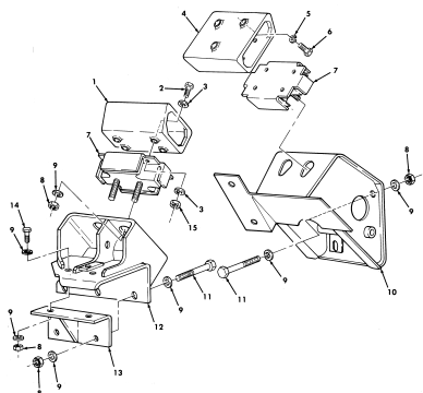
Figure 2. Engine Mounting Brackets.
