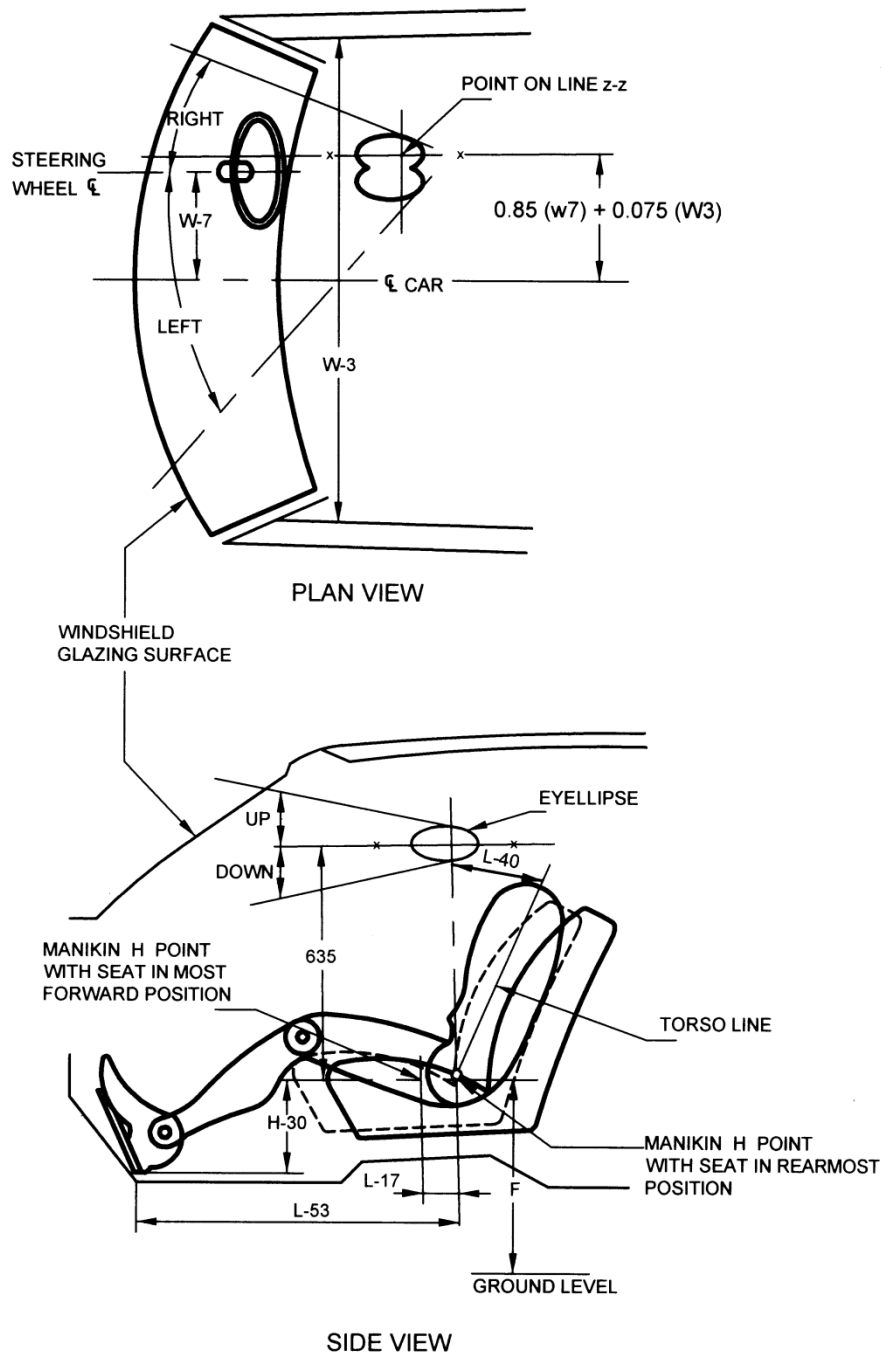
FIG. 1 EYELLIPSE TEMPLATE LOCATION FOR RIGHT HAND DRIVE
