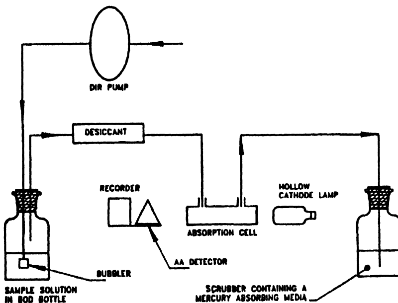
FIG. 1 SCHEMATIC ARRANGEMENT OF EQUIPMENT FOR MEASUREMENT OF MERCURY BY COLD VAPOUR ATOMIC ABSORPTION TECHNIQUE
