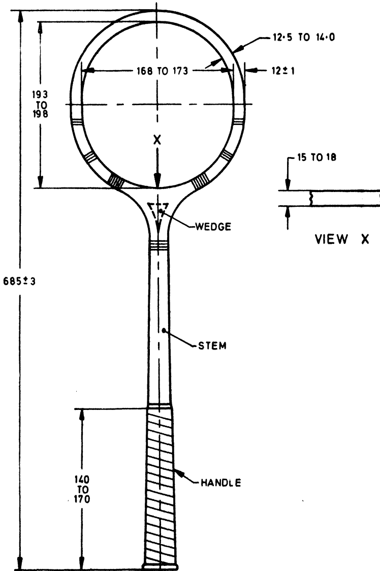
All dimensions in millimetres. FIG. 1 SQUASH RACKET FRAME
