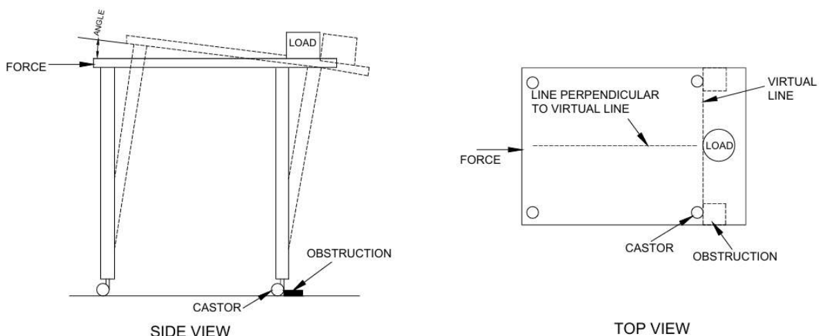
FIG. 3 HORIZONTAL STABILITY TEST
