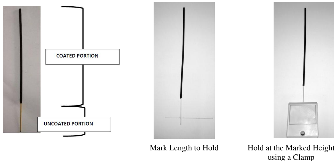
FIG. 1 TYPICAL REPRESENTATION OF CLAMPING ARRANGEMENT’
