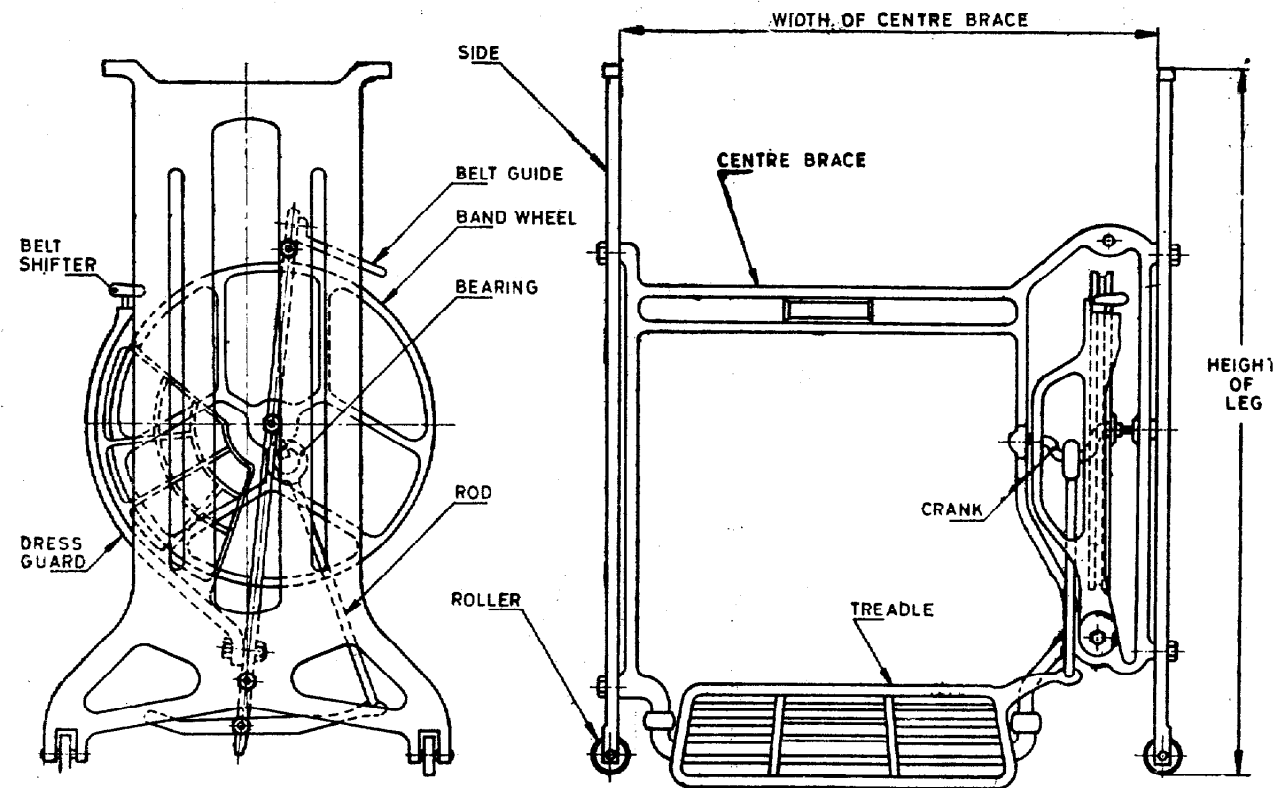
FIG. 1 NOMENCLATURE OF HOUSEHOLD SEWING MACHINE STAND ( TREADLE DRIVING EQUIPMENT )
