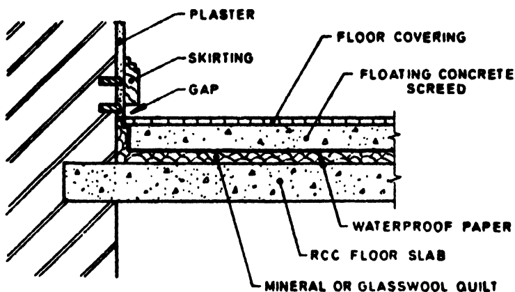
FIG. 3 CONCRETE FLOATING FLOOR CONSTRUCTION
