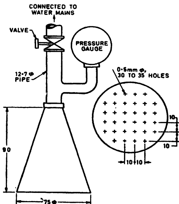
FIG. 1 WATER SPRAYER
