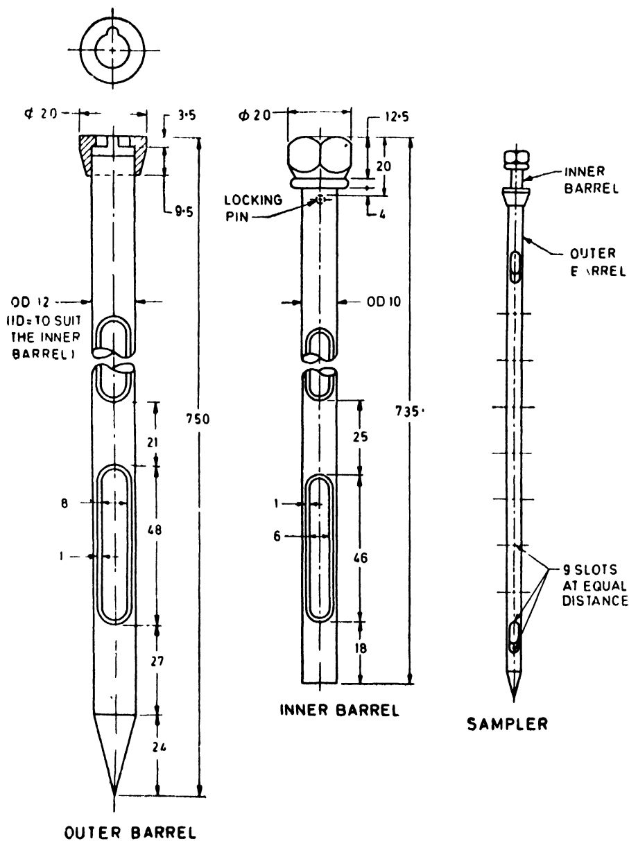
FIG. 1 TYPICAL SAMPLER FOR FORMULATIONS IN SOLID FORM ( AFDC 57 )
