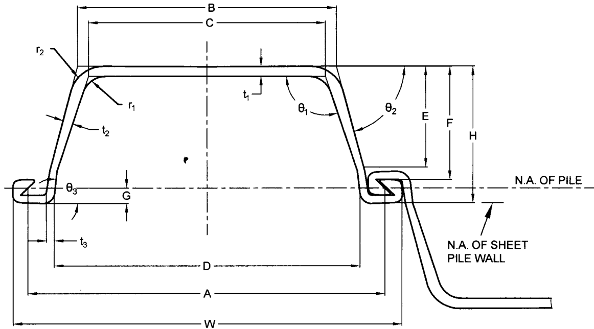
2A U-TYPE HOT ROLLED
