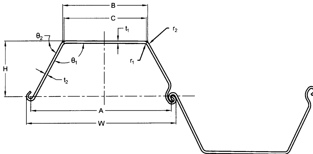
2B U-TYPE COLD FORMED
