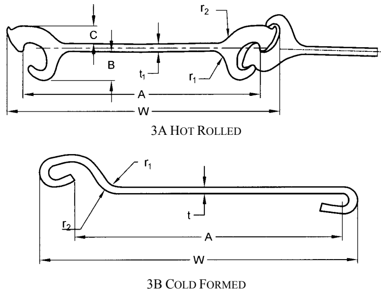
FIG. 3 FLAT-TYPE PILING SECTION
