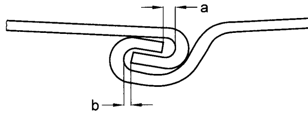
4B INTERLOCK DIMENSIONS, A AND B (COLD FORMED)
