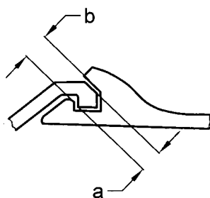
a = Button width b = Interlock opening, Z - type
