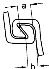
a = Hook width b = Interlock opening, U - type
