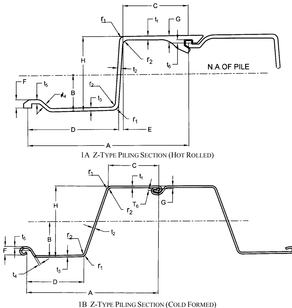
FIG. 1 Z-TYPE PILING SECTION
