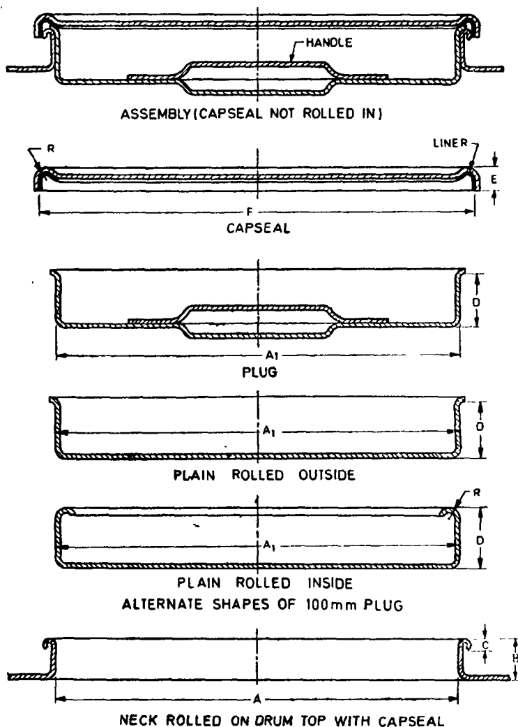
FIG. 2 INTEGRAL NECK WITH INNER LID AND CAPSEAL
