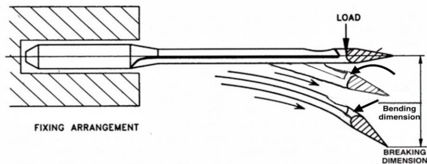
FIG. 1 ARRANGEMENT FOR BREAKING ANGLE TEST
