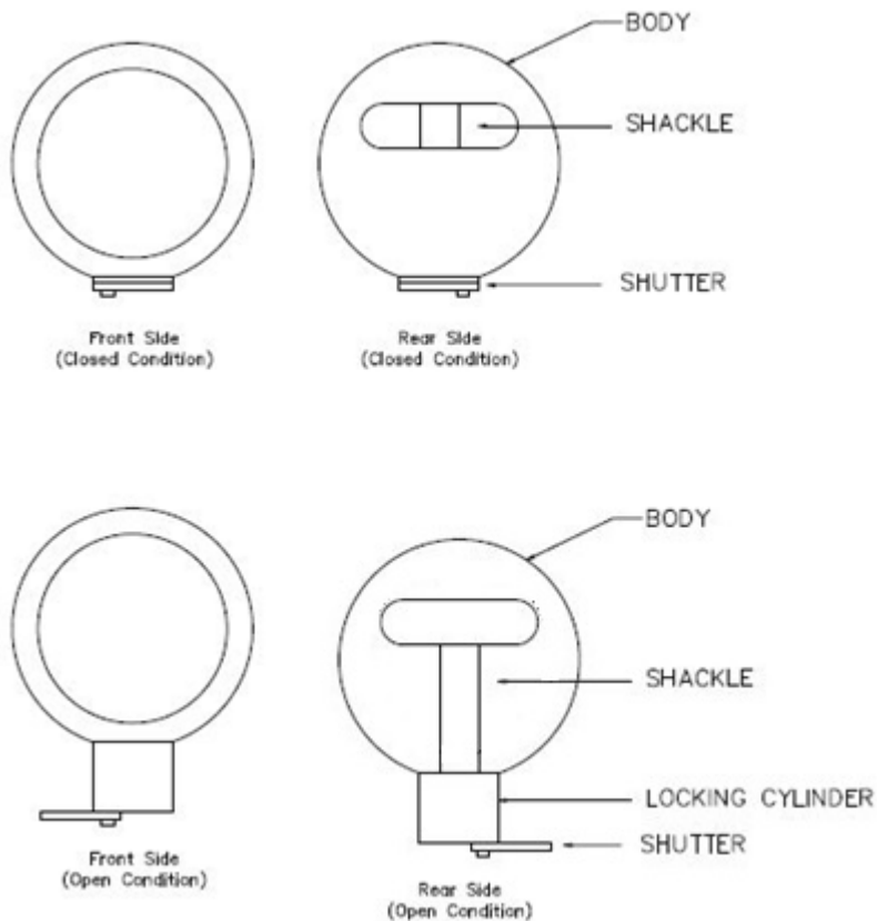
FIG. 8 CONCEALED SHACKLE PADLOCK'
