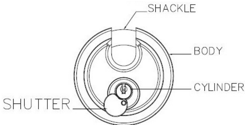
FIG. 7 CIRCULAR CLOSED SHACKLE PADLOCK
