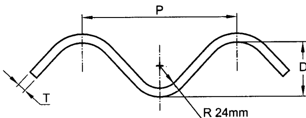
FIG. 1A PITCH AND DEPTH OF CORRUGATED SHEETS
