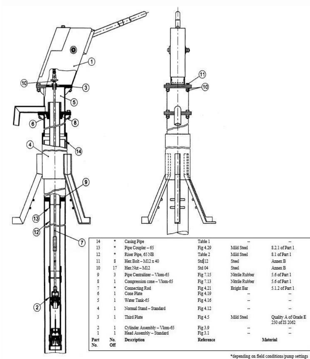
FIG. 2.2 DEEPWELL HANDPUMP - VLOM 65
