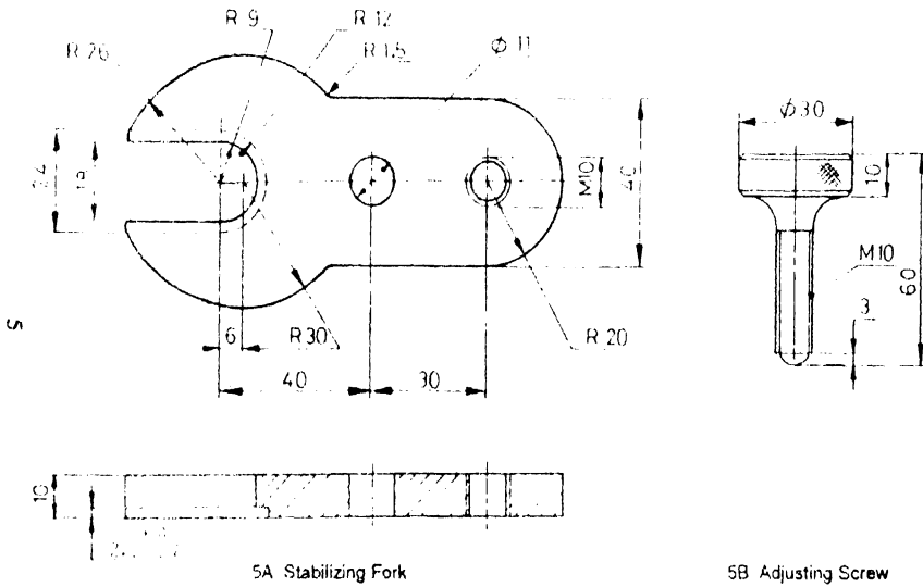
FIG. 5 ATTACHMENTS FOR FIXING THE CAPSULE
