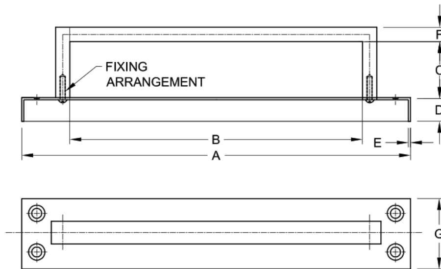
FIG. 5 TYPICAL DOOR HANDLE (TYPE 4)
