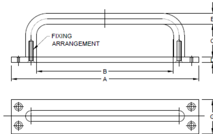
FIG. 4 TYPICAL DOOR HANDLE (TYPE 4)
