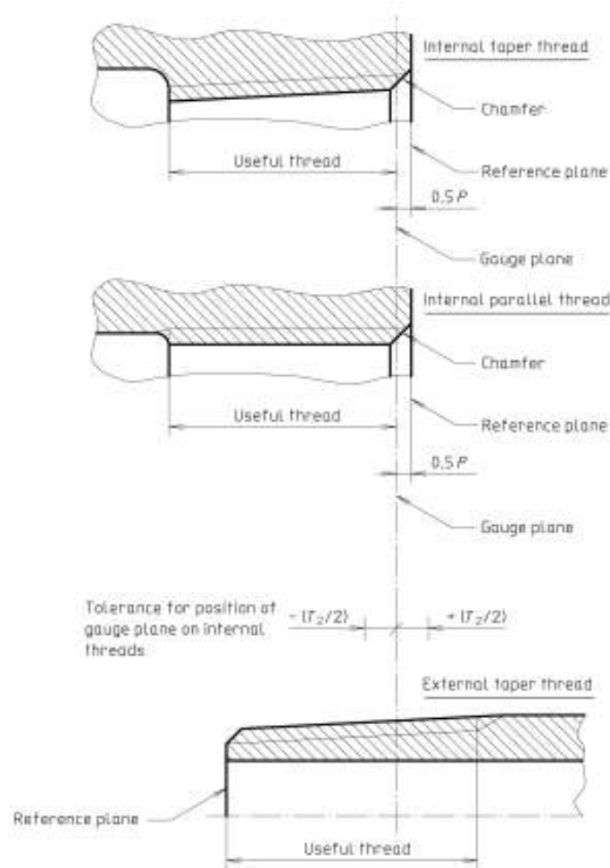
FIG. 5 ILLUSTRATION OF INTERNAL AND EXTERNAL PIPE THREADS (POSITION OF GAUGE PLANE, REFERENCE PLANE AND USEFUL THREAD)
