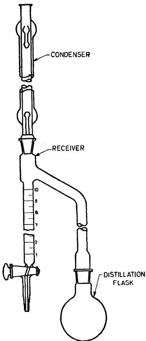
FIG. 1 TYPICAL ASSEMBLY OF APPARATUS FOR DETERMINATION OF MOISTURE
