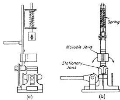
FIG. 9 APPARATUS FOR BEND TEST
