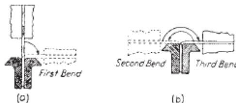
FIG.10 DIAGRAM ILLUSTRATING METHOD OF MAKING BENDS AND ARROWS INDICATE THE COUNT – STATING AS FIRST BEND, SECOND BEND ETC
