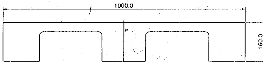
FIG. 4 INJECTION MOULDED PLASTIC PALLET FRONT VIEW
