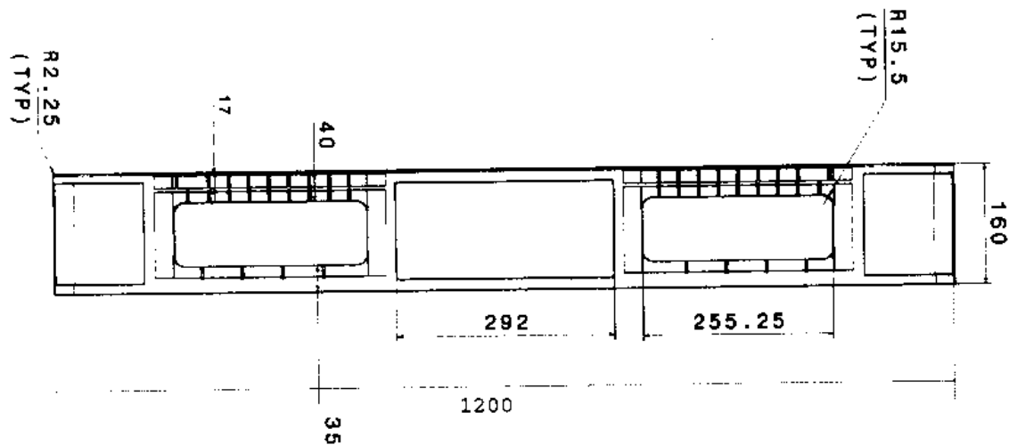
FIG. 3 STEEL REINFORCED INJECTION MOULDED PLASTIC PALLET SIDE VIEW
