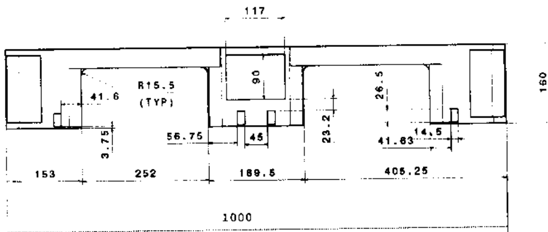
FIG. 2 STEEL REINFORCED INJECTION MOULDED PLASTIC PALLET FRONT VIEW
