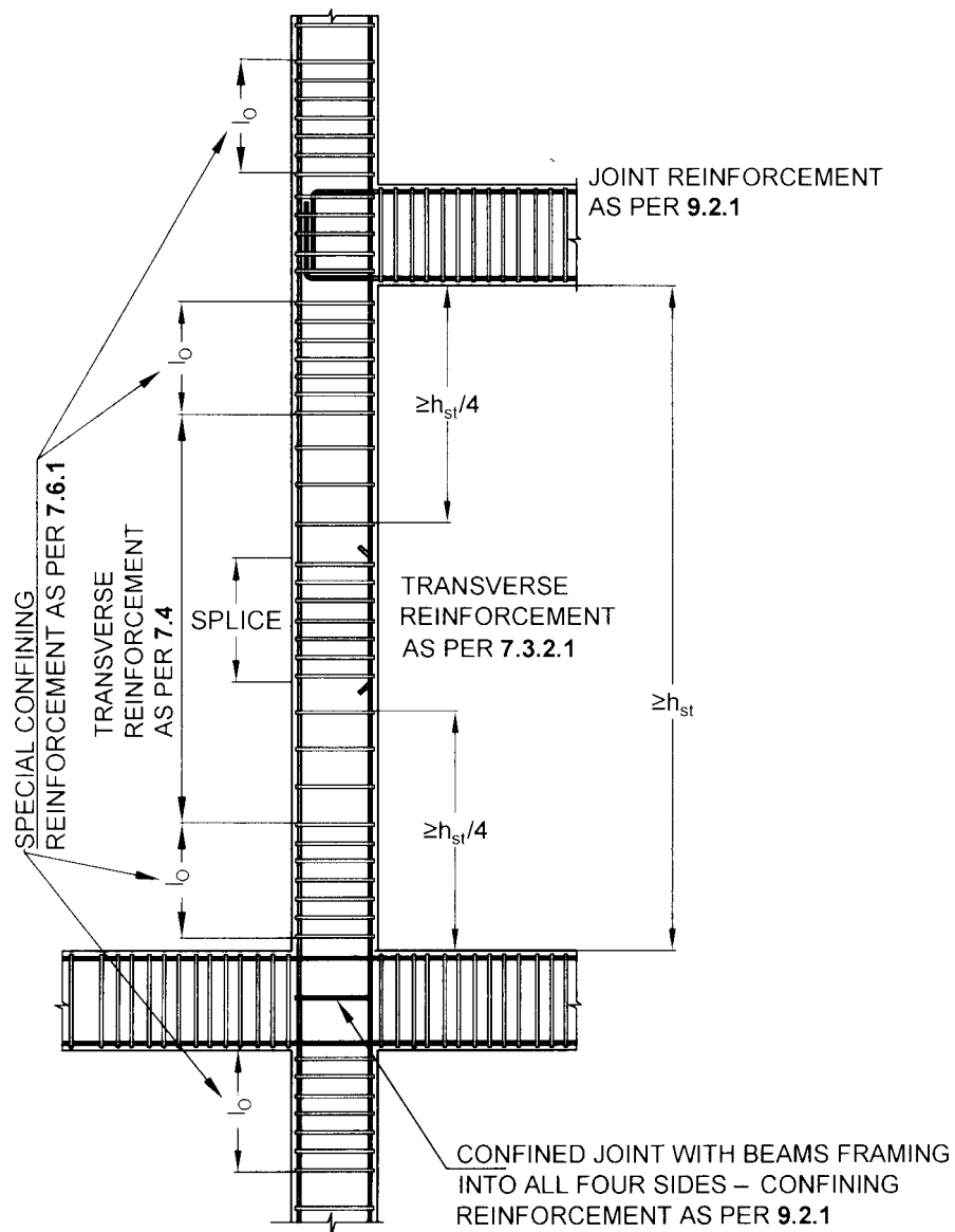
FIG. 12 COLUMNS AND JOINT DETAILING
