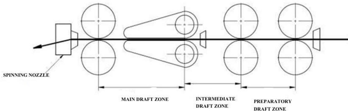
FIG. 33 4 OVER 4 SHORT DOUBLE APRON DRAFTING SYSTEM
