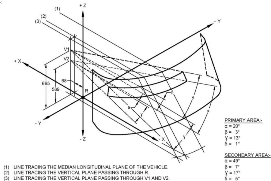
FIG. 2 VISION REQUIREMENTS IF STEERING WHEEL IS LOCATED TO RIGHT SIDE (PRIAMARY AREA)'
