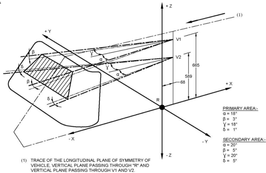
FIG. 1 VISION REQUIREMENTS IF STEERING WHEEL IS LOCATED CENTRALLY'
