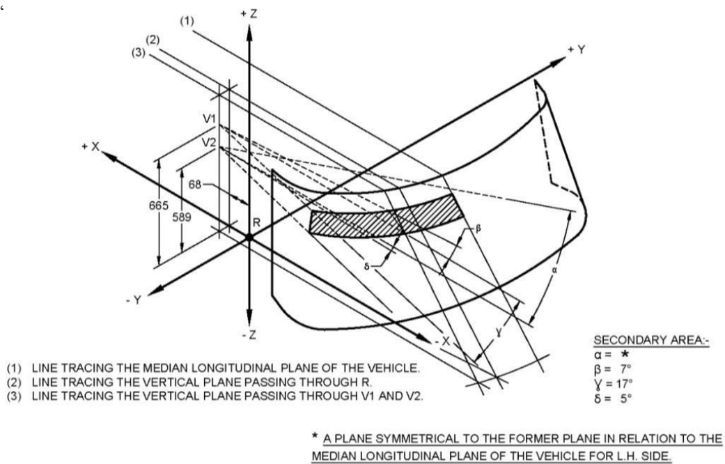
FIG. 3 VISION REQUIREMENTS IF STEERING WHEEL IS LOCATED TO RIGHT SIDE (SECONDARY AREA)*
