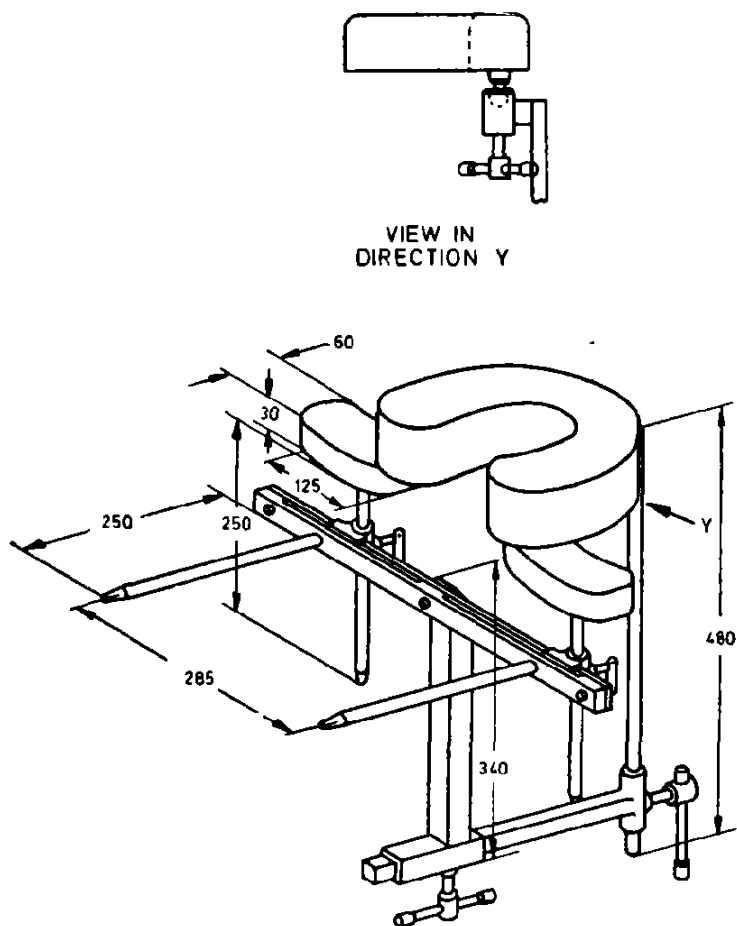
FIG. 2 NEUROSURGICAL ATTACHMENT FOR PRONE POSITION HEAD-REST
