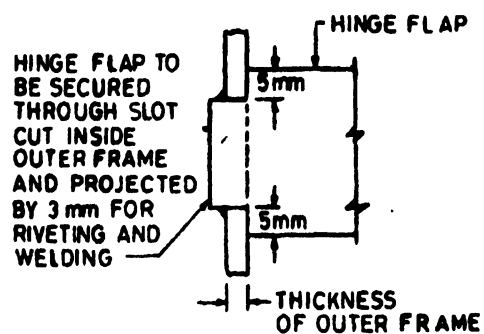
DETAIL AT A
