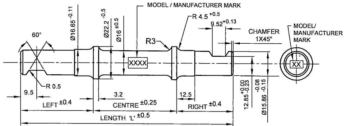
FIG. 1 COTTERED BOTTOM BRACKET AXLE
