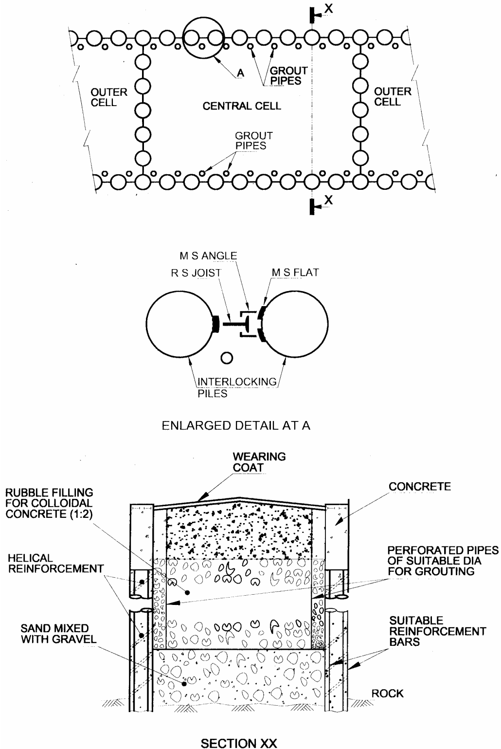
FIG. 1 COLLOIDAL CONCRETE COFFER DAMS
