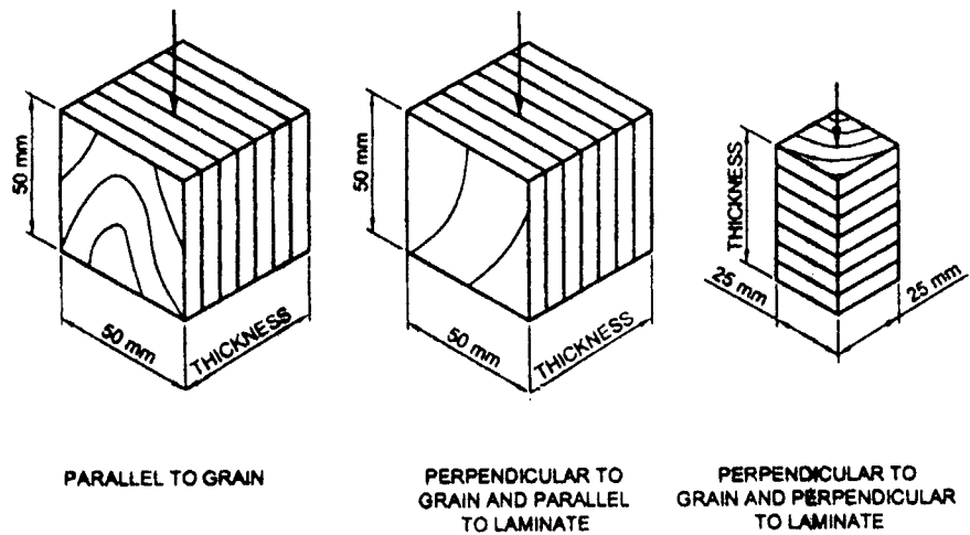
FIG. 1 PLACEMENT OF FORCES FOR COMPRESSIVE STRENGTH
