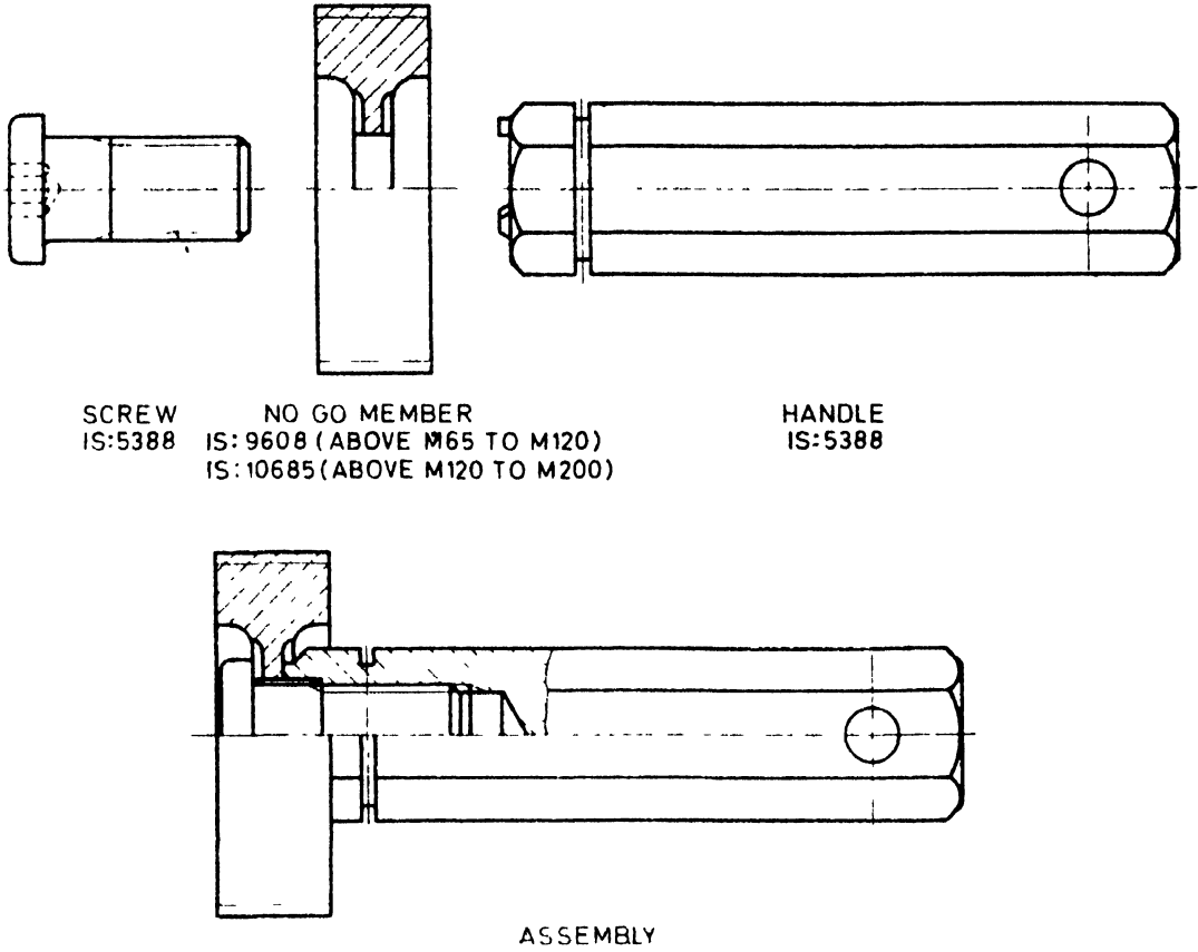
FIG. 5B NO GO SCREW GAUGE ASSEMBLY FOR NOMINAL SIZE ABOVE M65 UP TO AND INCLUDING M200
