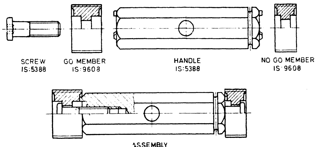
FIG. 4 GO AND NO GO SCREW GAUGE ASSEMBLY FOR NOMINAL SIZE ABOVE M40 UP TO AND INCLUDING M65 ( Pages 2 and 3, Figs. 5A and 5B ) — Substitute the following for the existing figures:
