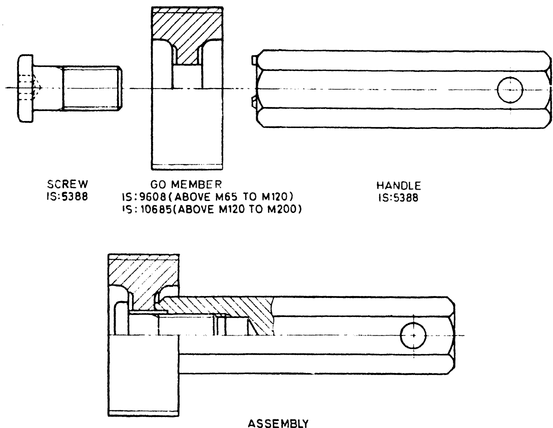
FIG. 5A GO SCREW GAUGE ASSEMBLY FOR NOMINAL SIZE ABOVE M65 UP TO AND INCLUDING M200
