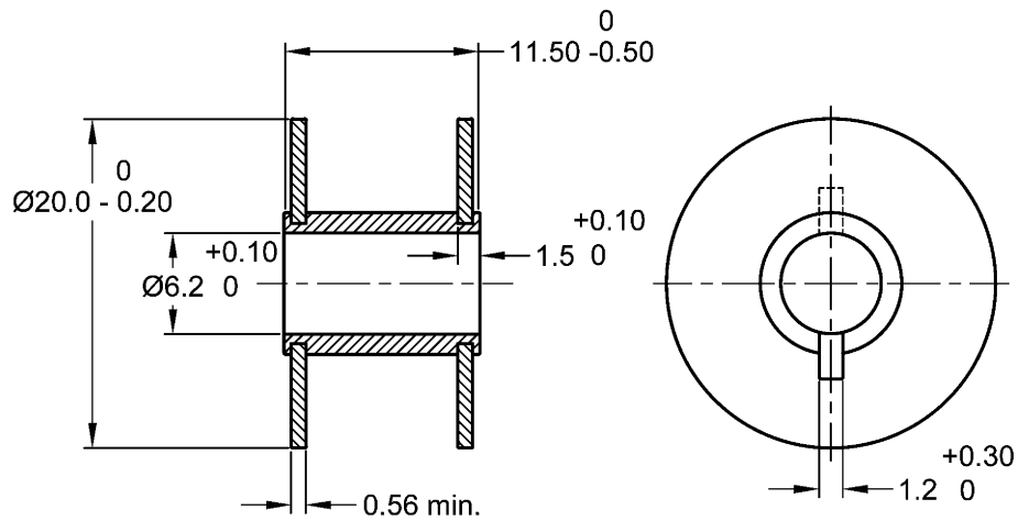
FIG. 2 DIMENSIONS FOR BOBBINS
