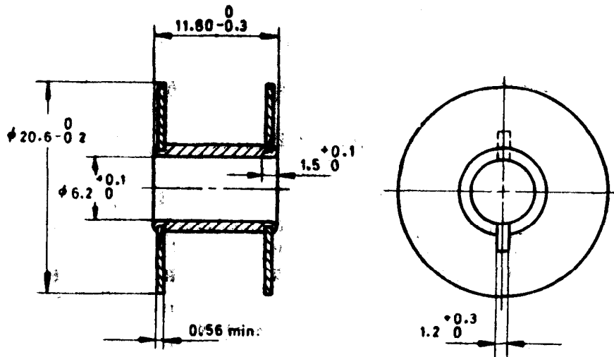
FIG. 2 DIMENSIONS FOR BOBBINS
