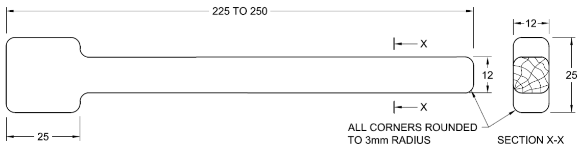
All dimensions in millimetres. FIG. 3 POKING ROD
