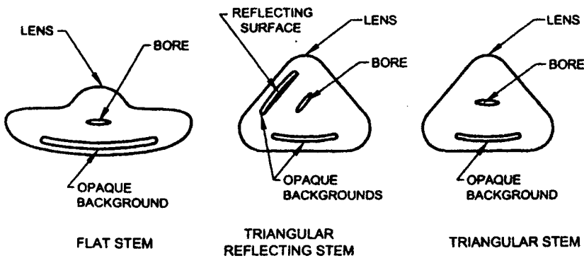
FIG. 1 CROSS SECTION OF MAGNIFYING LENS STEMS
