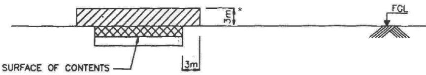
FIG. M8B DISSOLVED AIR FLOATATION (DAF) UNITS (APPLICABLE FOR OPEN TANKS OR BASINS)
