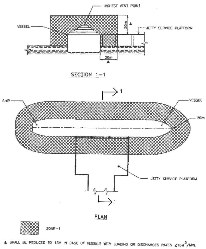
FIG. M10 JETTIES OR MARINE FACILITIES
