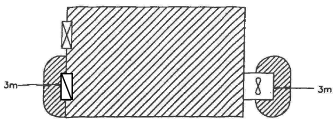
FIG. M9C FLAMMABLE SUBSTANCES RELEASED DURING ABNORMAL SITUATION OR INFREQUENT OPERATIONS WITH ADEQUATE VENTILATION
