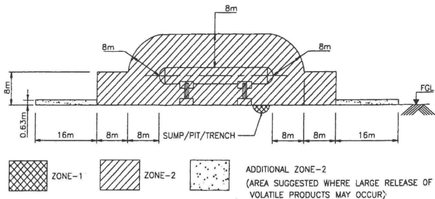
FIG. H9 PRESSURE STORAGE TANK (BULLET) (HEAVIER-THAN-AIR GASES OR VAPOUR)
