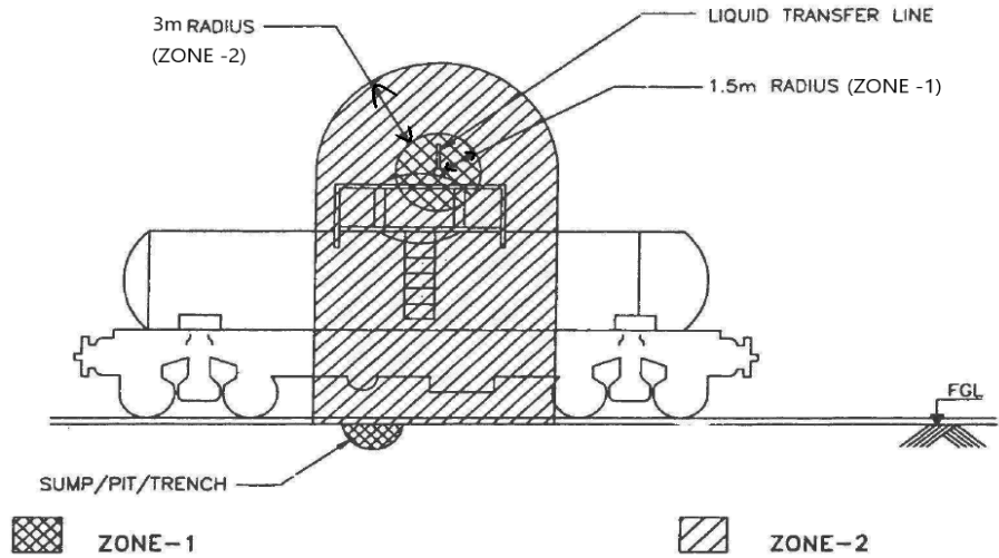
FIG. M3B (MATERIAL: FLAMMABLE LIQUID) WAGON/TANK TRUCK LOADING AND UNLOADING VIA OPEN SYSTEM. TOP OR BOTTOM PRODUCT TRANSFER
