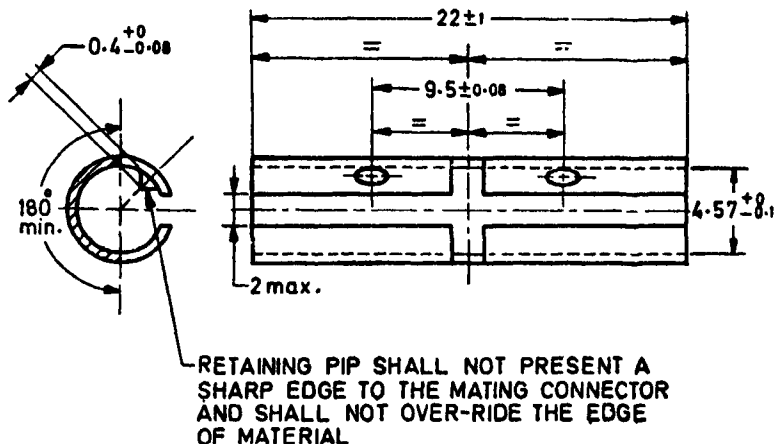
FIG. 2. TUBE TYPE CONNECTOR
