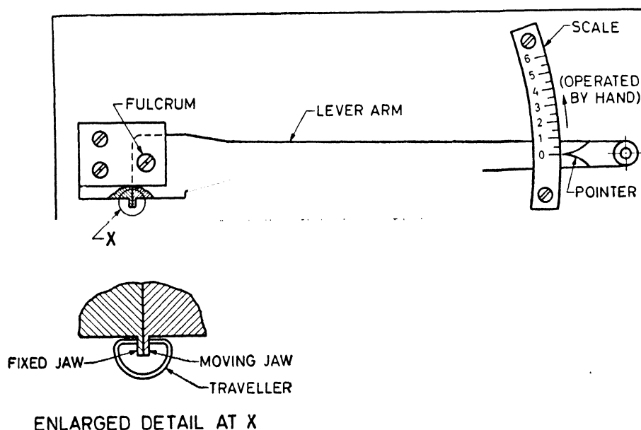
FIG. 2 A TYPICAL STRETCH TESTING APPARATUS FOR TRAVELLERS
