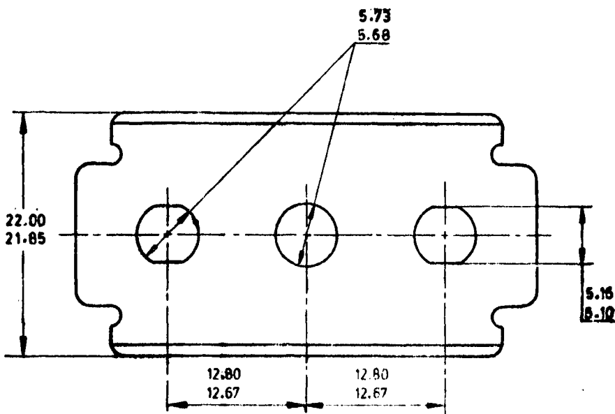
FIG. 3 STAINLESS STEEL SAFETY RAZOR BLADE PIN TYPE
