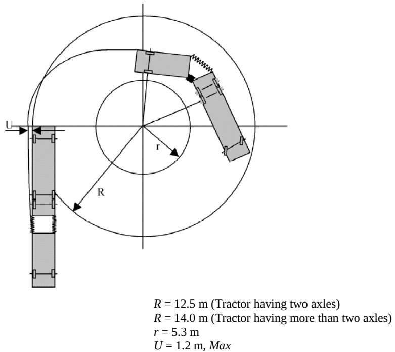
FIG. 2 MANEUVERABILITY FOR ARTICULATED VEHICLES
