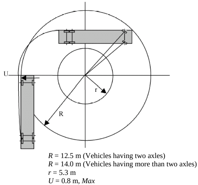
FIG. 1 MANEUVERABILITY FOR RIGID VEHICLES
