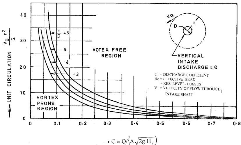
7A FOR VERTICAL INTAKES
