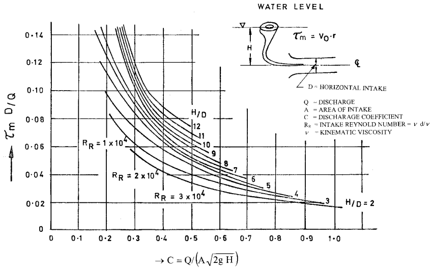
FIG. 7 DIAGRAMS FOR DETERMINING OPTIMUM SUBMERGENCE
