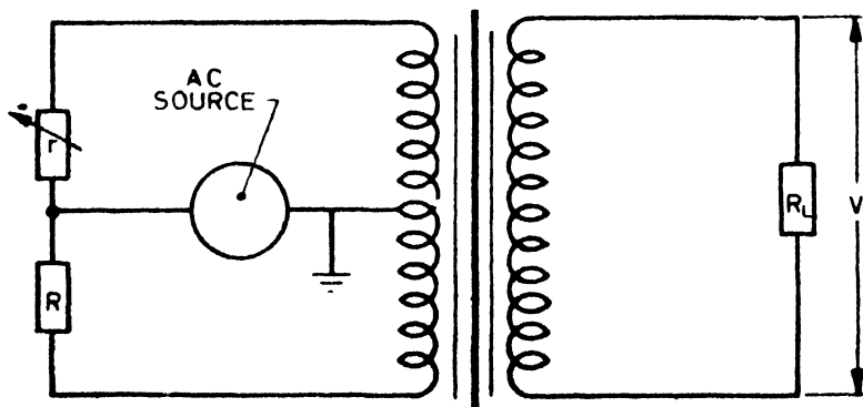
FIG. 2 ARRANGEMENT FOR CENTRE TAP BALANCE TEST
